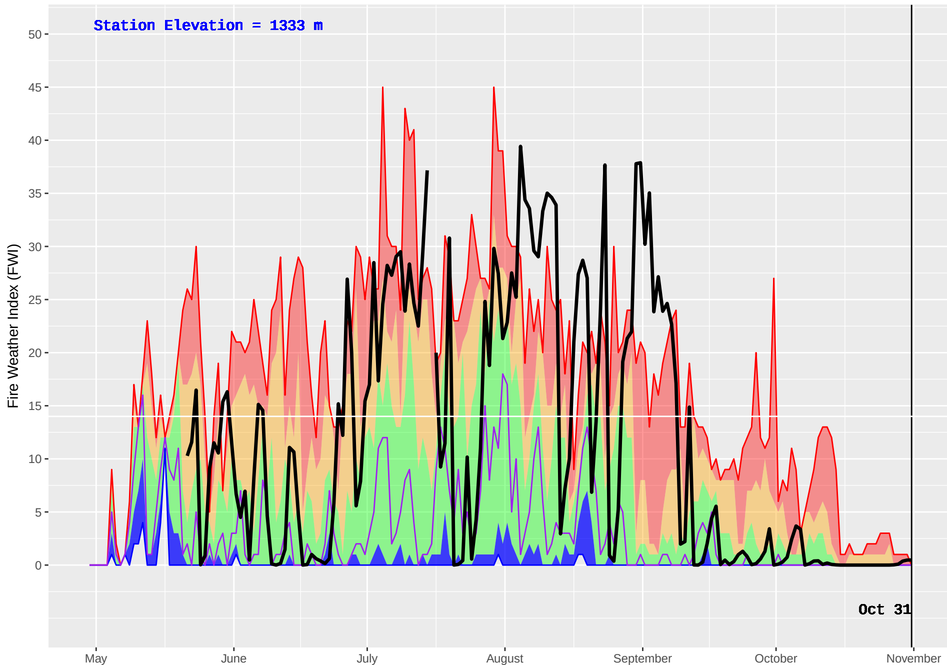
GOLDSTREAM 2 (919) : Historical (2005–2016) and Current (2017) Noon Fire Weather Index (FWI)
