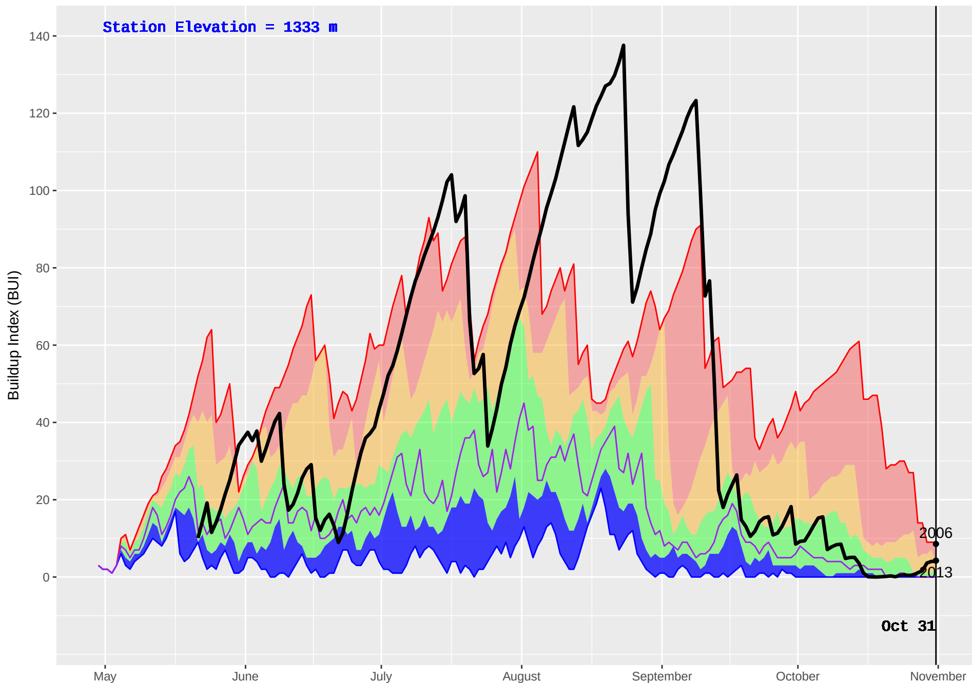
GOLDSTREAM 2 (919) : Historical (2005–2016) and Current (2017) Noon Buildup Index (BUI)
